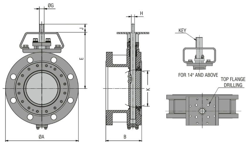
Double Flanged Body
